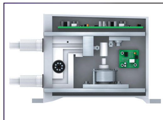
Model U802 CUTAWAY
