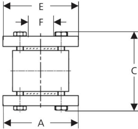
Dimensions Sleeve Connection [mm]
