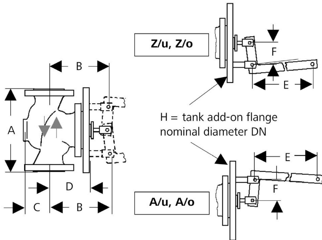
Dimensions [mm] and Weights [kg] PN 10/16*
