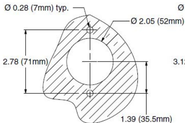
STANDARD PANEL MOUNT CUT OUT
