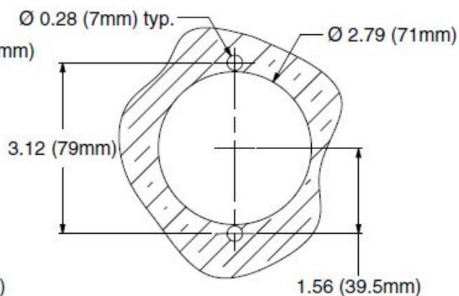
CAPTURED VENT PANEL MOUNT CUT OUT
