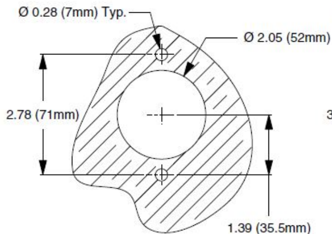
STANDARD PANEL MOUNT CUT OUT
