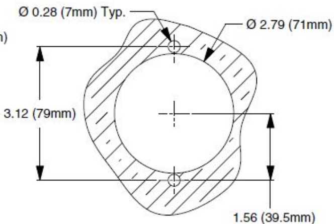
CAPTURED VENT PANEL MOUNT CUT OUT
