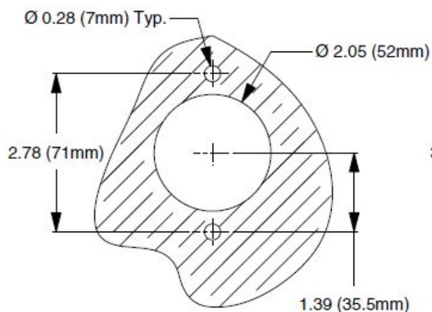
STANDARD PANEL MOUNT CUT OUT
