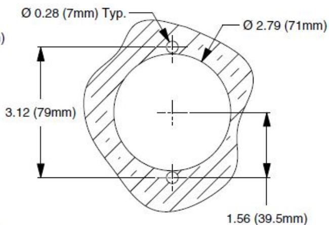
CAPTURED VENT PANEL MOUNT CUT OUT
