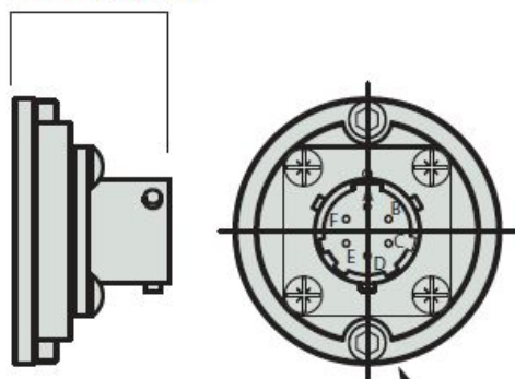
SECTION A
